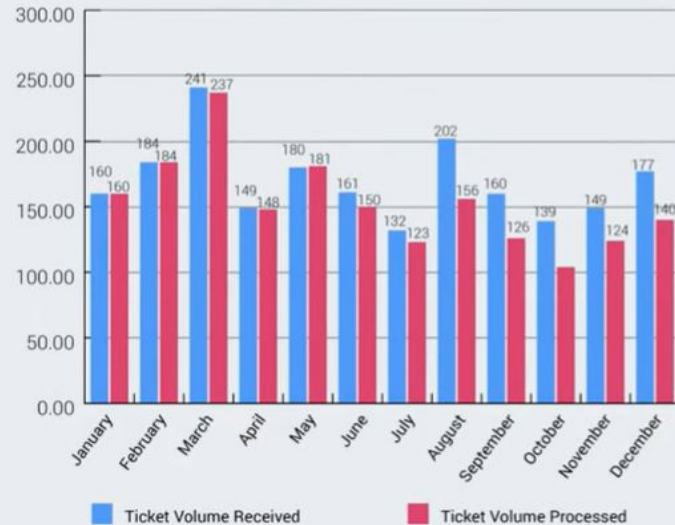
TICKET TREND
